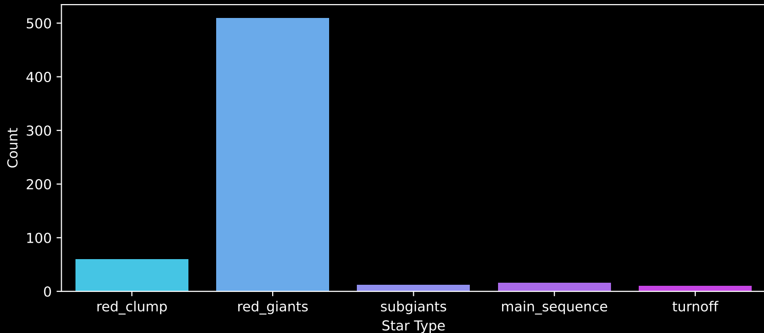
APOGEE DR17 Field: [M22] Count plot of Star Type
