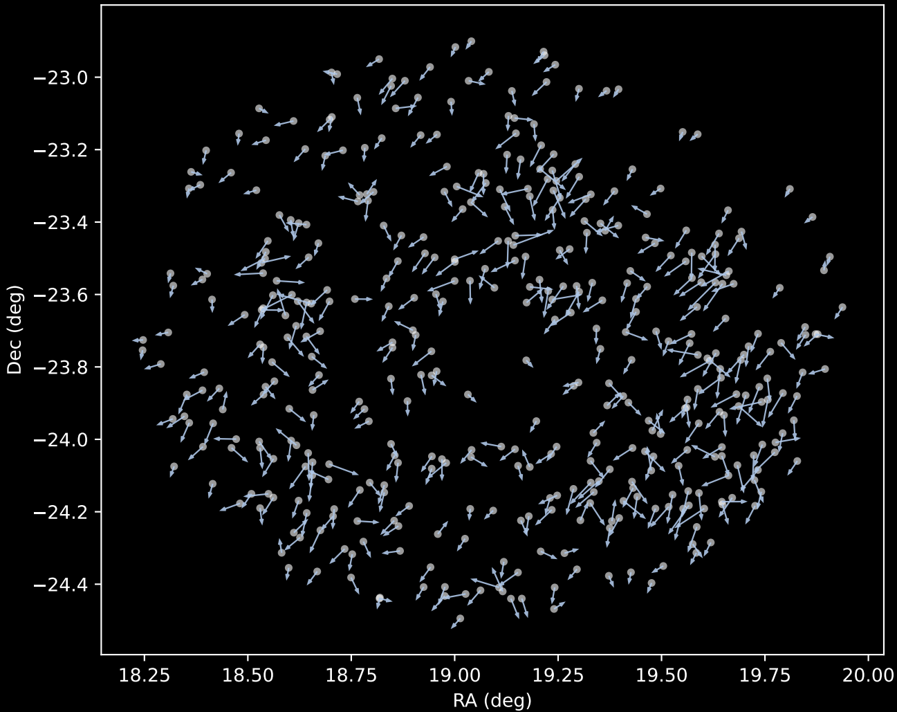
APOGEE DR17 Cluster 1 Proper Motion Vectors (n=429)
