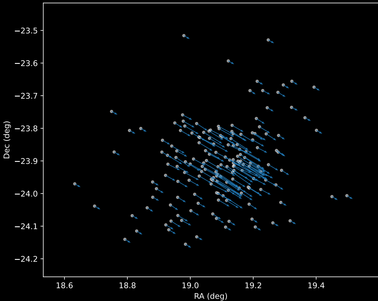
APOGEE DR17 Cluster 0 Proper Motion Vectors (n=164)
