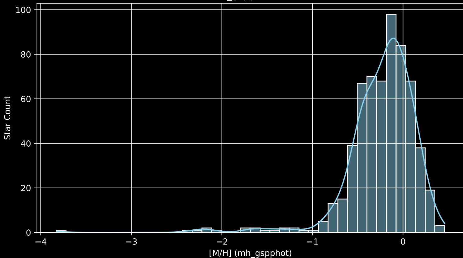
APOGEE DR17 Field: [M22 [M/H] (mh_gspphot) (n= 605)
