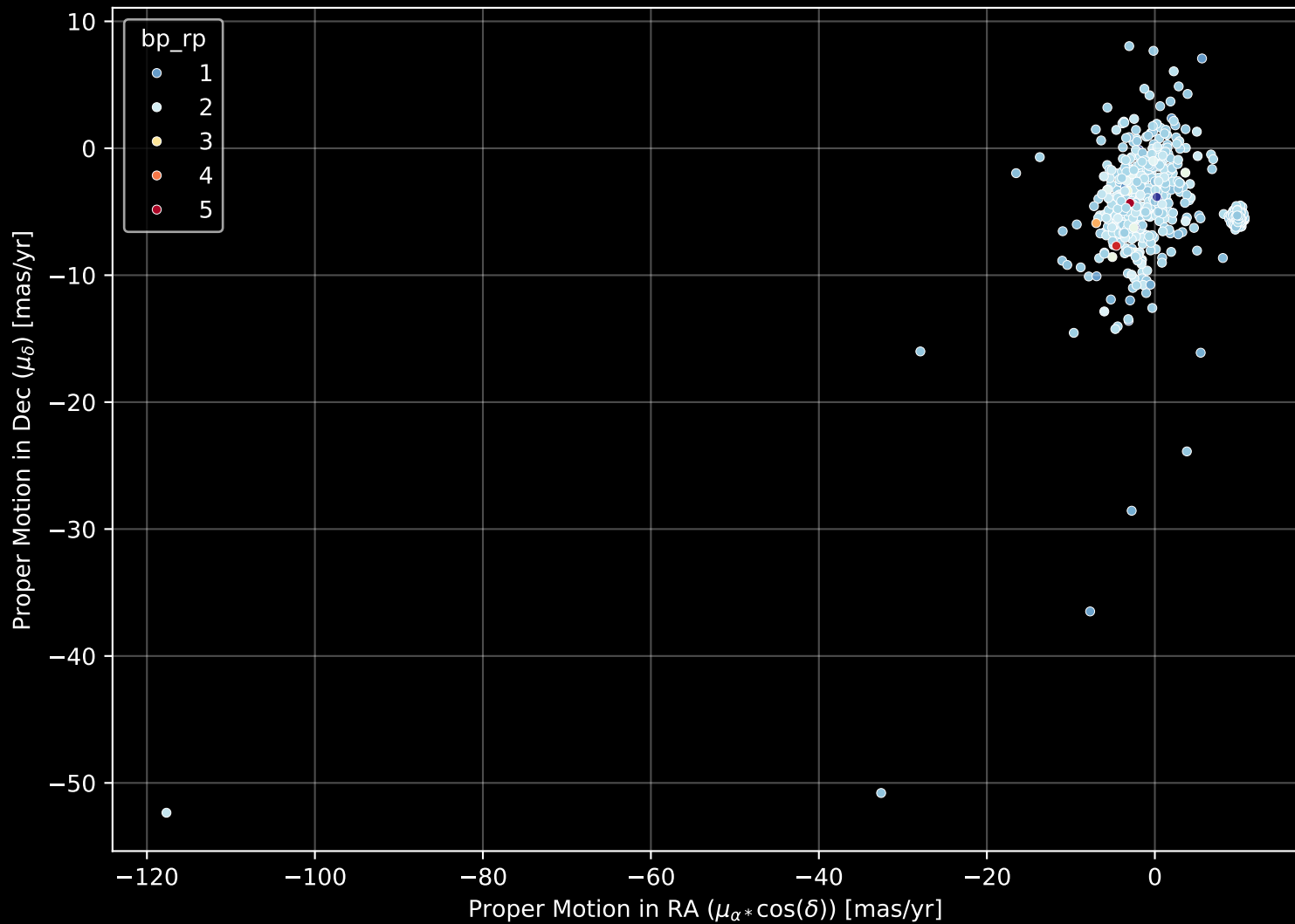
APOGEE DR17 Field: [M22] Proper Motion Diagram (n= 607)
