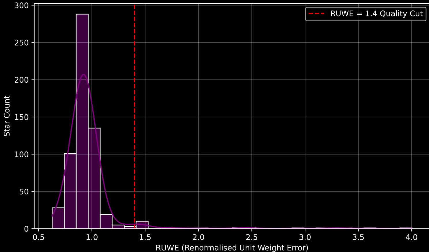
GAPOGEE DR17 Field [M22] RUWE Distribution (n= 604)
