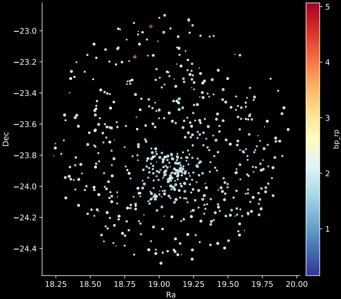
APOGEE DR17 Field: [M22] Stars: 607
