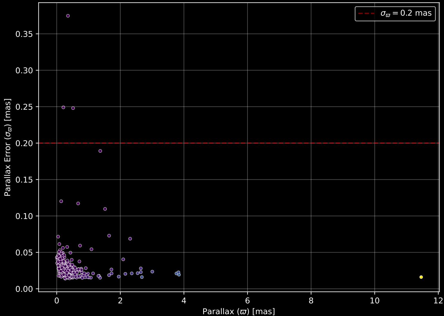
APOGEE DR17 Field: [M22] Parallax Quality (n= 607)
